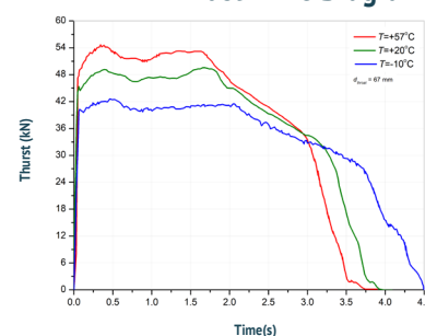
Thrust-Time Diagram
