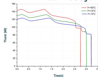
Thrust-Time Diagram
