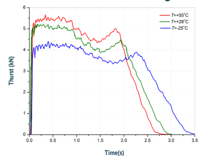
Thrust-Time Diagram
