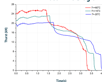
Thrust-Time Diagram
